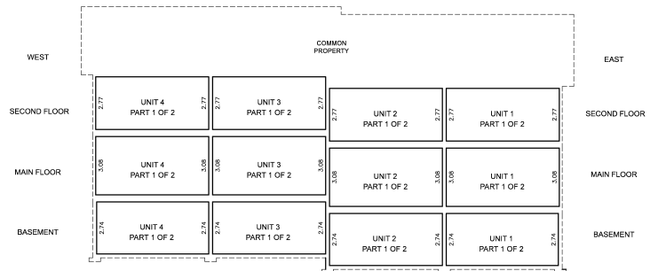
CROSS-SECTION A-A'
